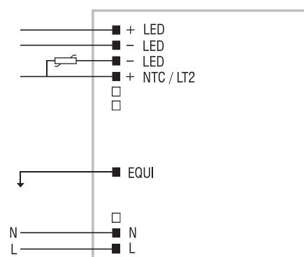
MIDNIGHT diagram Collegamento MIDNIGHT
